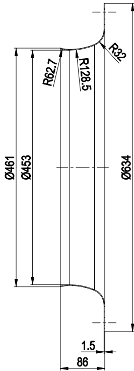
Inlet ring 63300-2-4013
